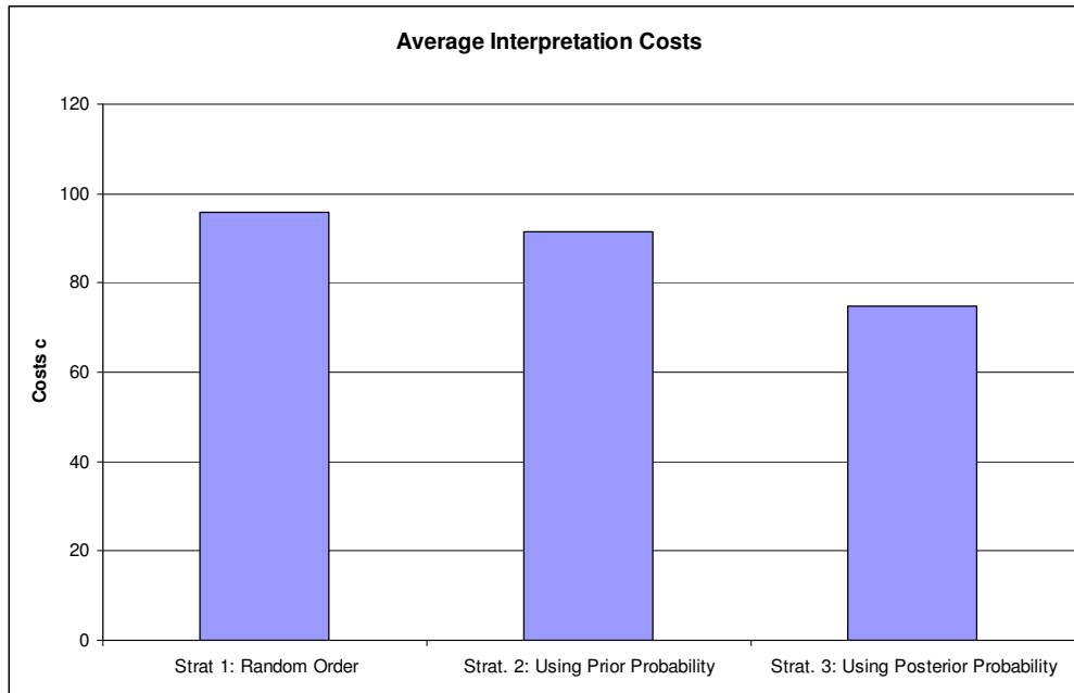
Fig. 6: Simulated average interpretation costs for different image interpretation strategies (taken from the article “Probabilistic reasoning on object occurrence in complex scenes” 11 ). The costs represent the effort to create a complete scene description. Strategy 3 uses the proposed inference method to adaptively search for object classes with a high occurrence probability. Strategy 2 merely uses the prior occurrence probability, without incorporating intermediate detections of objects. Strategy 1 randomly selects object classes to search for.
